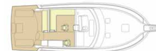
STANDARD HELM DECK ARRANGEMENT
