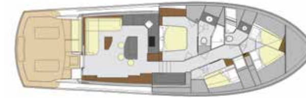
INTERIOR WITH OPTIONAL TACKLE CENTER, BOW STATEROOM AND CENTER ISLAND GALLEY
